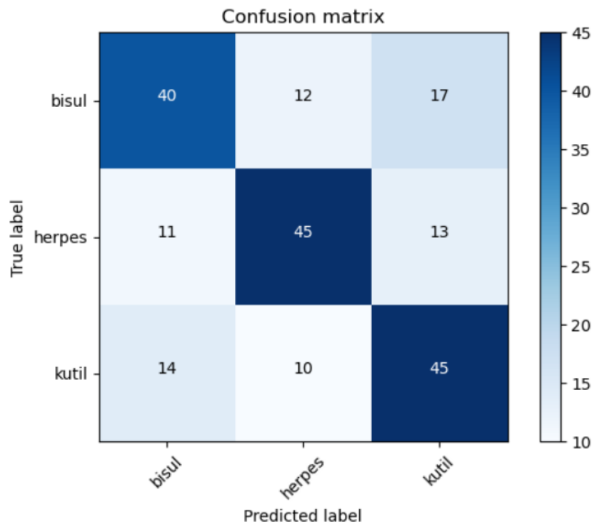
Fig. 4. Confusion Matrix
